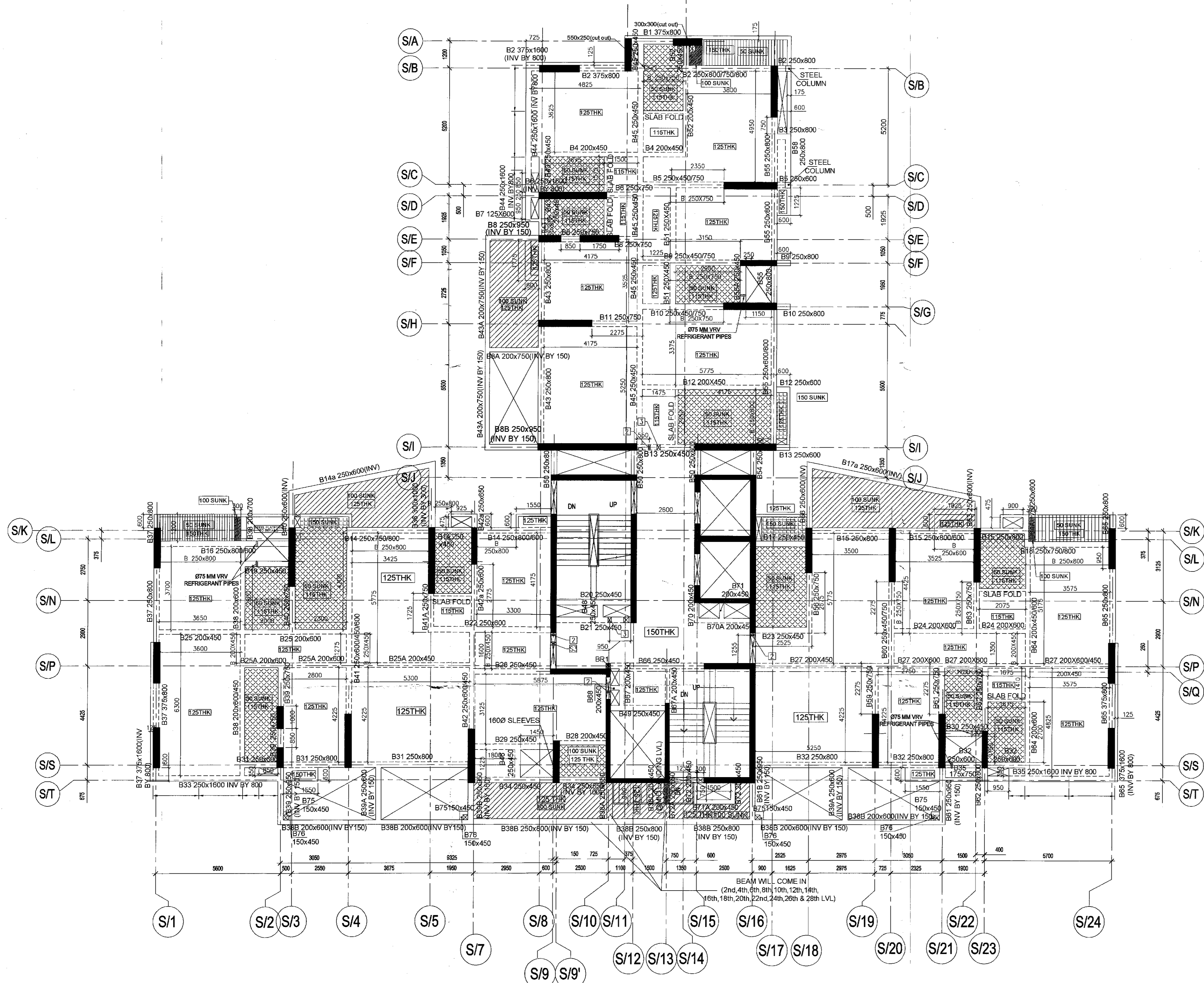
TYP. FL SHUTTERING LAYOUT (2ND-27TH)
